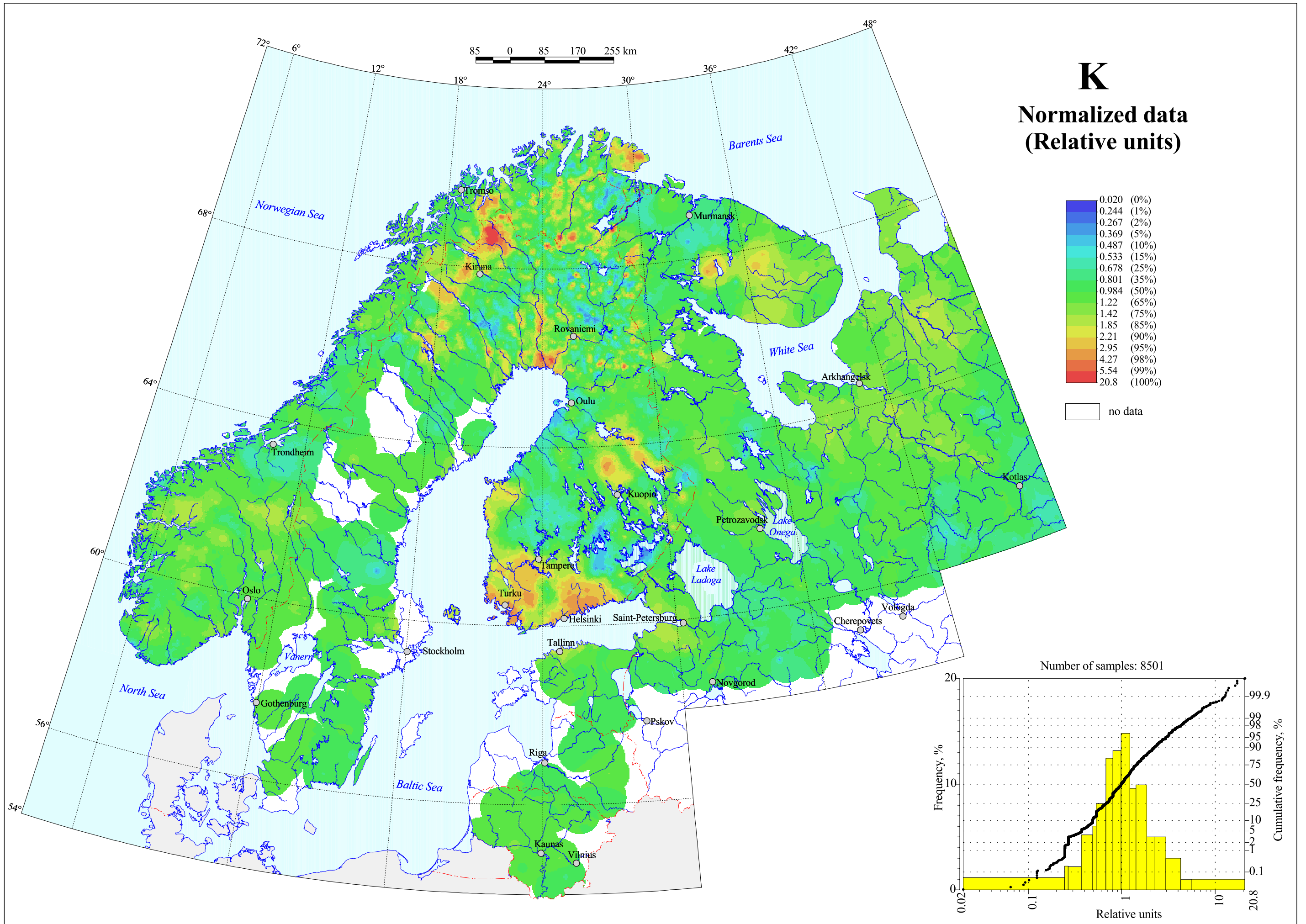
Potassium in Stream Sediment
